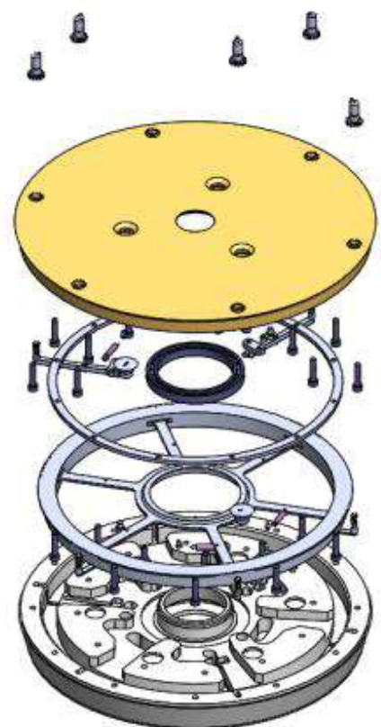
12" Lam Spin Base 853-109087-262 853-109087-201
